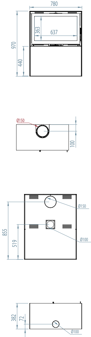
MODUL-ART 77 woodbox
