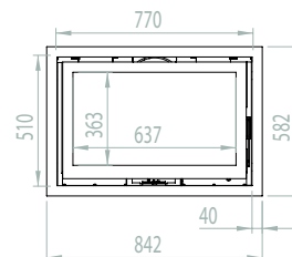
PURE 77/51
