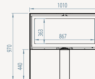
VENTIL-ART 16/9 woodbox
