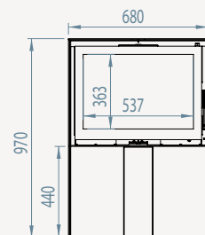
VENTIL-ART 67/51 woodbox
