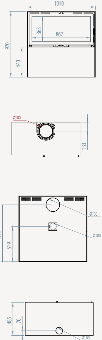
MODUL-ART 16/9 woodbox
