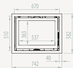
PURE 67/51
