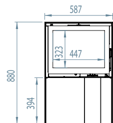
VENTIL-ART 58/47 woodbox
