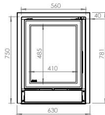
NORDIC PLUS 56/75
